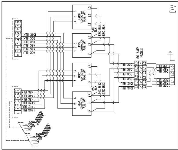
8051633A EPR/TRIAC TERMINAL BLOCK WIRING DIAGRAMS 8051634B 22kW TERMINAL BLOCK WIRING DIAGRAMS 8051652C SINGLE PHASE TERMINAL BLOCK WIRING DIAGRAMS
