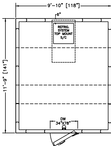
PLAN VIEW
