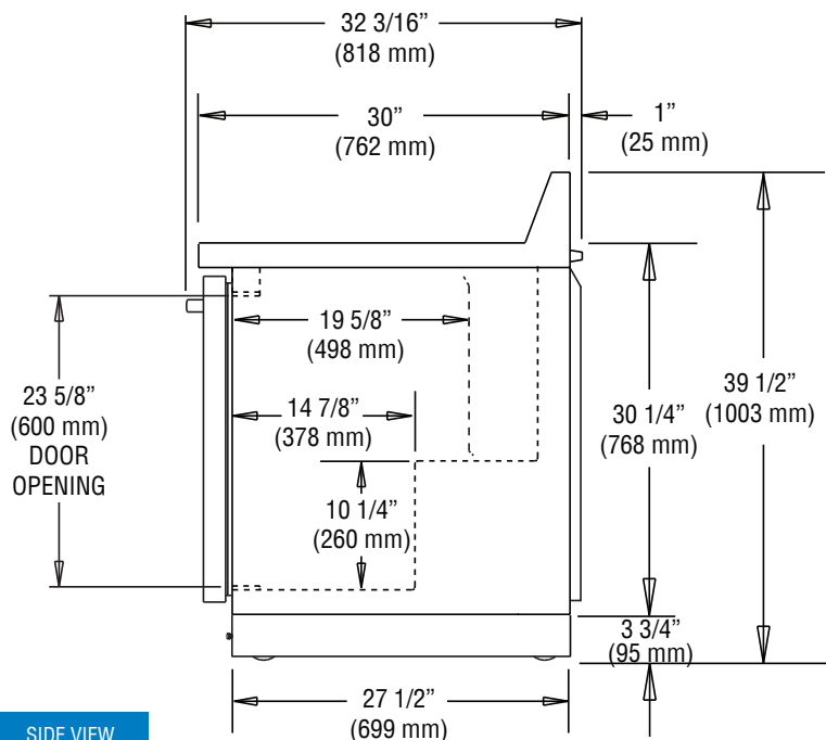
SIDE VIEW
