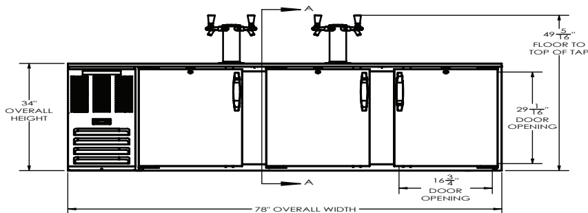
ELEVATION VIEW
