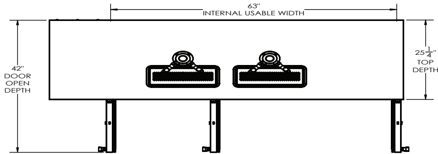
ELEVATION VIEW
