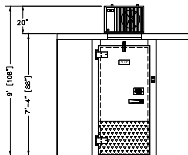
ELEVATION LEFT HINGE
