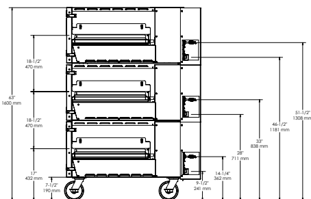
2424 Gas Triple Stack Side View
