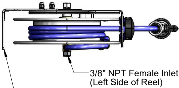
Open Stainless Steel Hose Reel; 35' of 3/8" Hose
