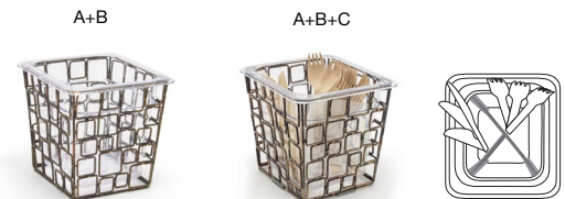
A 1/6 Size Pan - Deep pack 4 BHO054CLT21 6.75 x 6.25 x 5.75 in, 2.25 qt | 17.3 x 16 x 14.6 cm, 2.1 L B 1/6 Size Coppered Link Housing - Deep pack 4 BHO051GOI21 6.25 x 5.75 x 6 in | 15.6 x 14.4 x 15.2 cm A+B 1/6 Size Coppered Link Housing/Pan Set - Deep pack 4 BHO061GOI21 6.75 x 6.25 x 6 in, 2.25 qt | 17.3 x 16 x 15.2 cm, 2.1 L C Flatware Divider Insert pack 4 BHO077FRT21 6.5 x 3.25 x 3.75 in | 16.3 x 8.1 x 9.5 cm A+B+C 1/6 Size Coppered Link Flatware Divider Set pack 4 BHO078GOI21 6.75 x 6.25 x 6 in | 17.3 x 16 x 15.2 cm Shown with: Servewise® Utensils See on page 145
