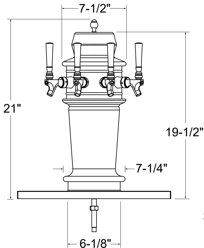
FRONT ELEVATION
