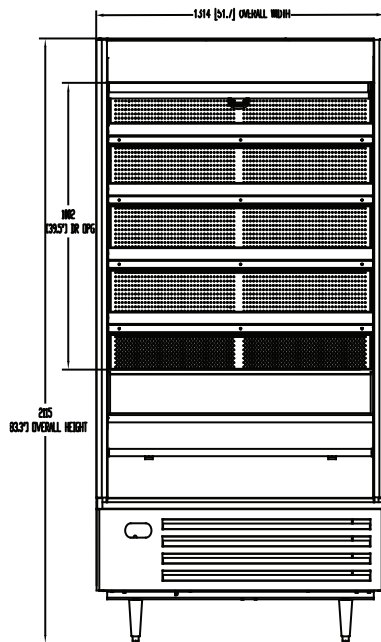
ELEVATION VIEW
