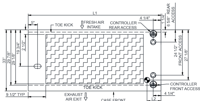
PLAN VIEW
