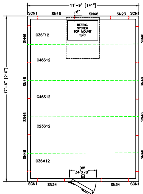
PLAN VIEW LEFT HINGE SELECT
