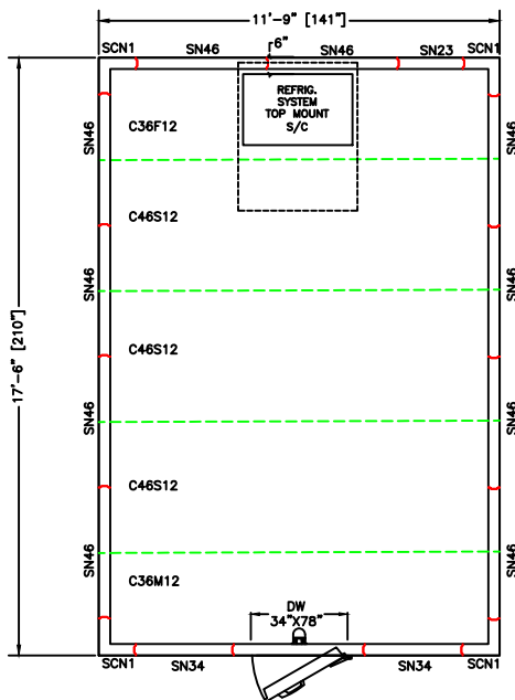
PLAN VIEW RIGHT HINGE SELECT
