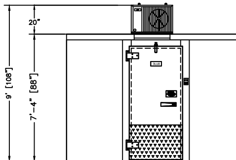
ELEVATION LEFT HINGE
