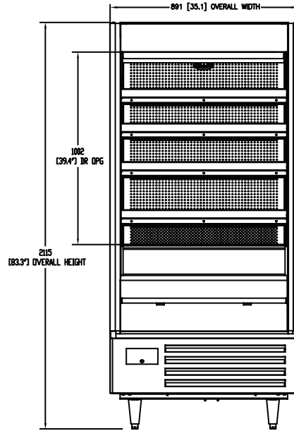
ELEVATION VIEW
