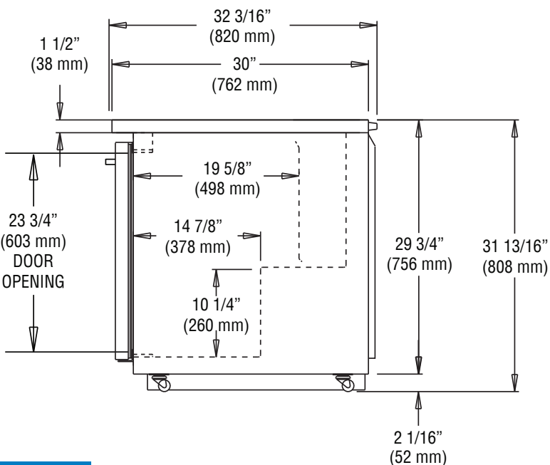
SIDE VIEW
