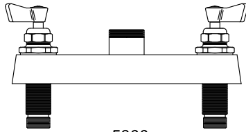
5300 CONTROL VALVE
