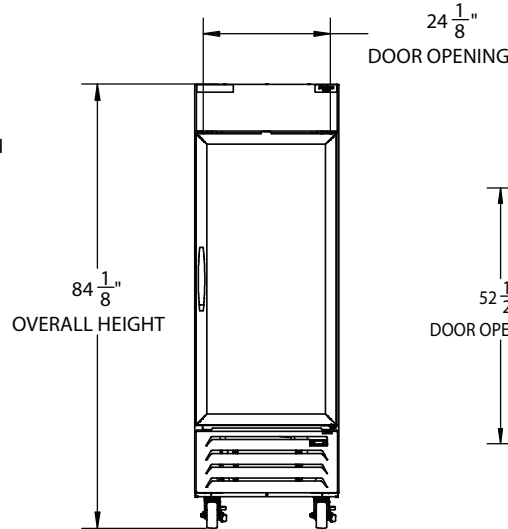
ELEVATION VIEW
