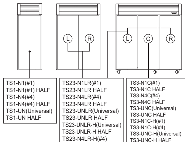
TS1-N1(#1) (9) pairs #1 tray slides and pilasters
