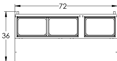
Top Configuration
