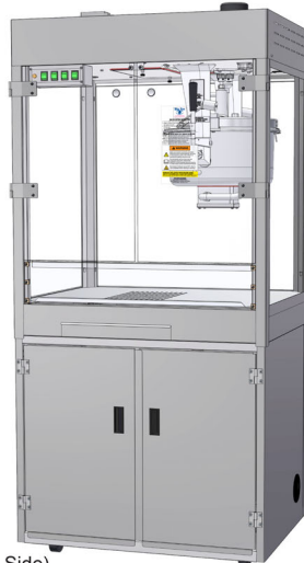
2671 (841) Counter Model Front Counter (Customer Side)
