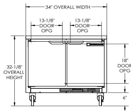
ELEVATION VIEW
