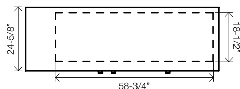
FBB-24-72(G)(S)-HC Top View
