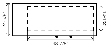
FBB-24-60(G)(S)-HC Top View
