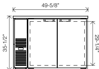
FBB-24-48(G)(S)-HC Front View
