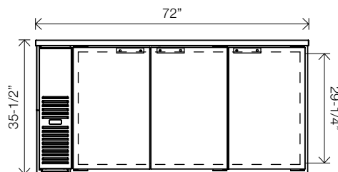
FBB-24-72(G)(S)-HC Front View
