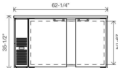
FBB-24-60(G)(S)-HC Front View
