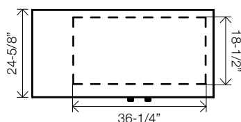
FBB-24-48(G)(S)-HC Top View
