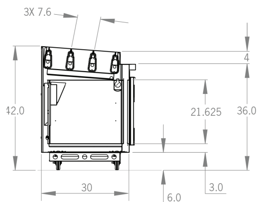
Section View
