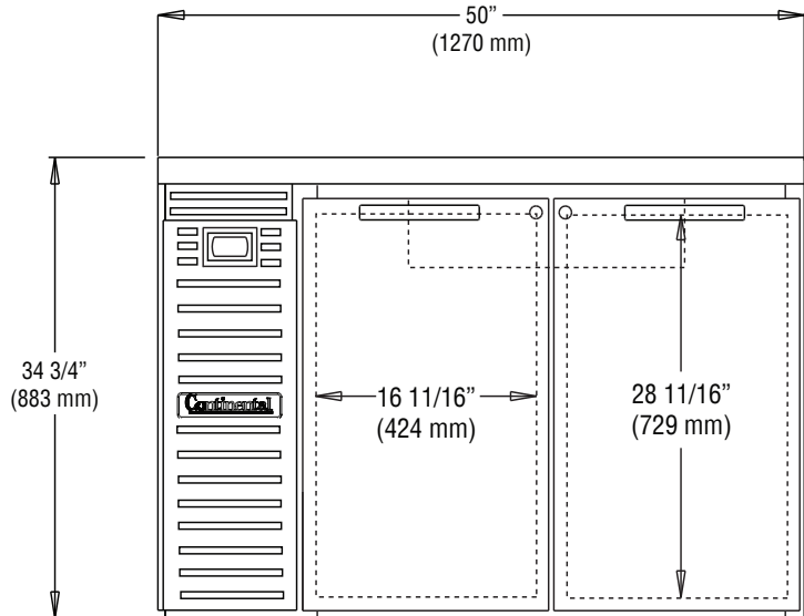
FRONT VIEW
