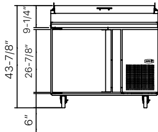
FPT-46 Front View
