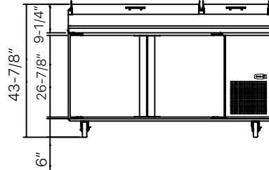
FPT-67 Front View
