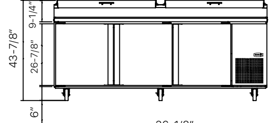
FPT-93 Front View
