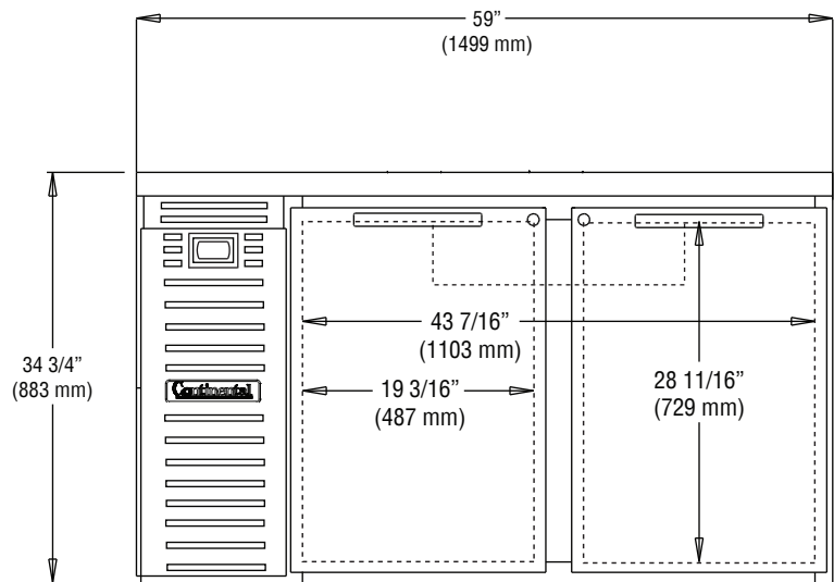
FRONT VIEW
