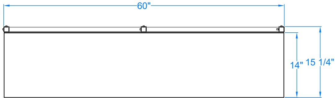
Top View
