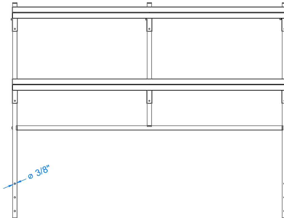
Front View
