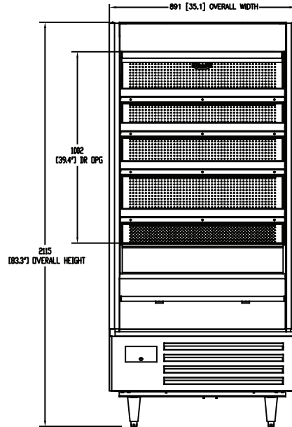
ELEVATION VIEW
