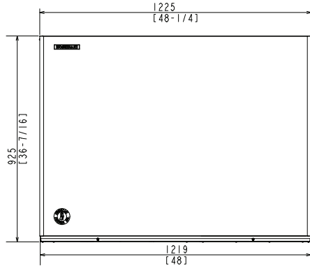
WATER-COOLED
