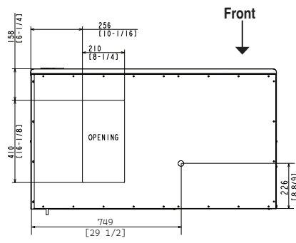
REMOTE AIR-COOLED
