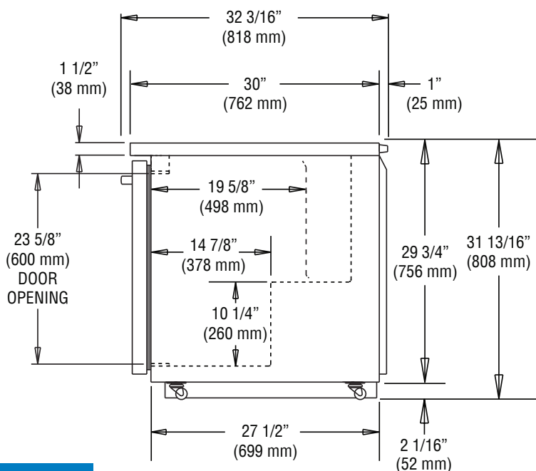
SIDE VIEW
