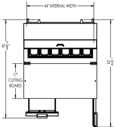
PLAN VIEW
