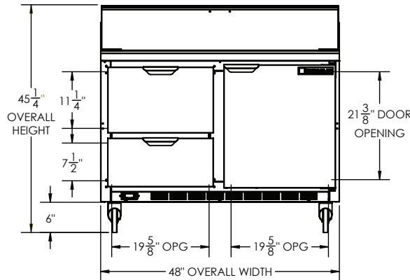
ELEVATION VIEW
