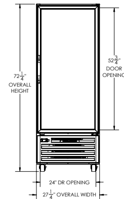
ELEVATION VIEW
