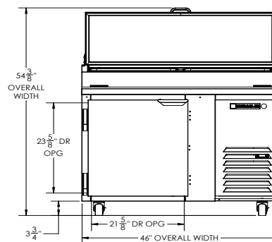
ELEVATION VIEW
