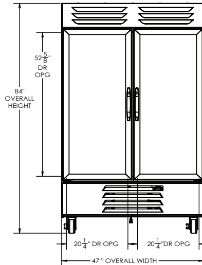
ELEVATION VIEW
