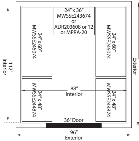
AWC0810-TF-EL/ER
