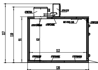
AWC0808-TF-EL/ER
