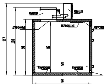
AWC0606-TF-EL/ER
