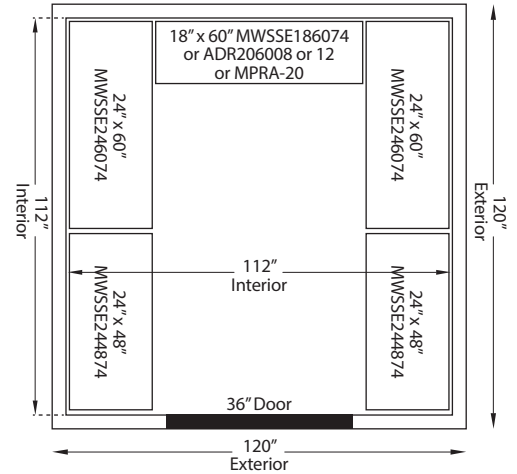
AWC1010-TF-EL/ER
