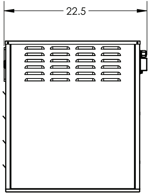
Right Side View: Model MHD42SSL1T
