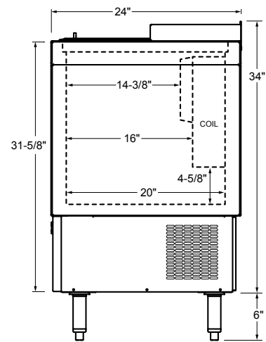
SIDE ELEVATION
