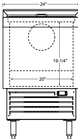
FRONT ELEVATION
