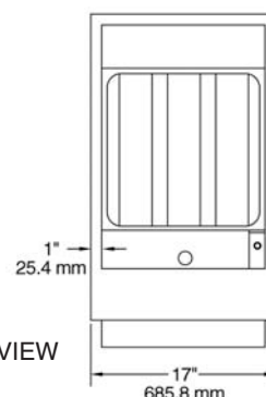
CUTOUT FOR COUNTER TOP
