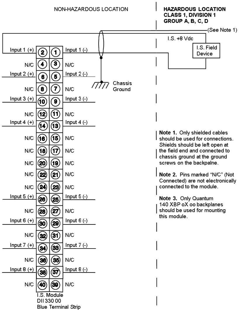
31001365 Rev 00 140 DII 330 00 Wiring Diagram
