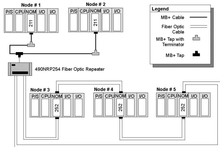
Self-Healing Ring Configuration Example
