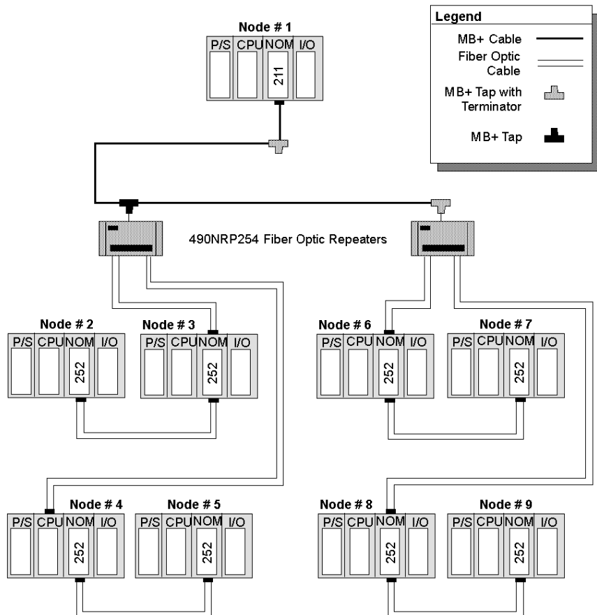
Tree Configuration Example
