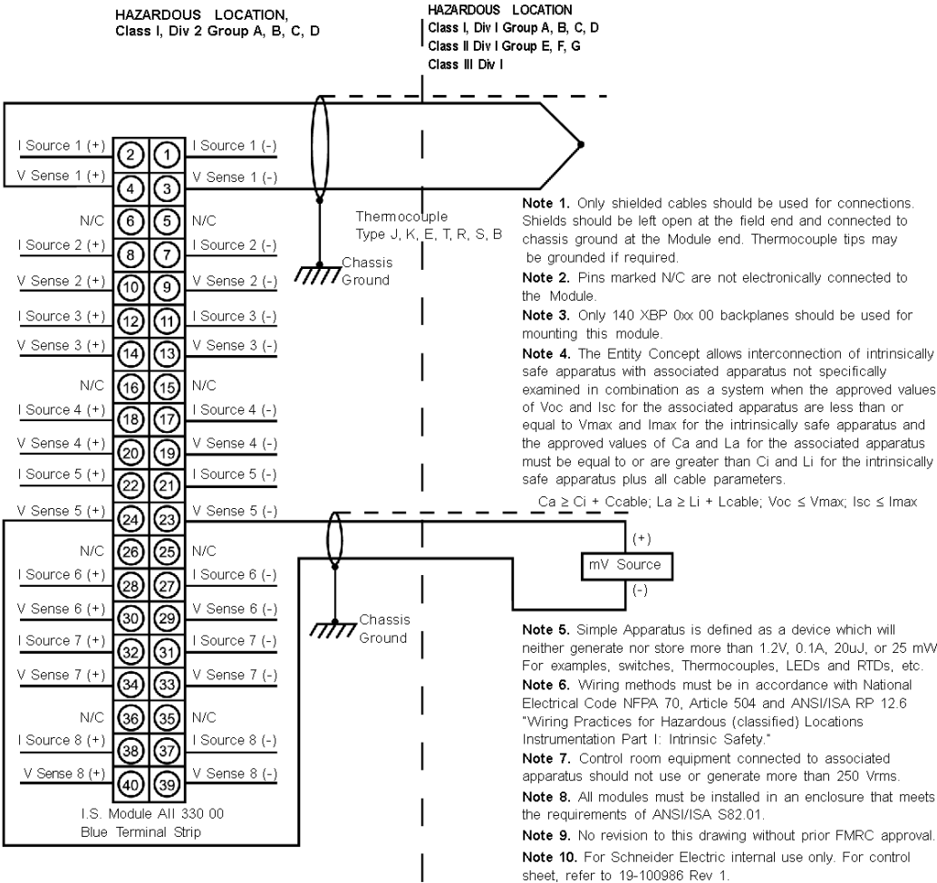
140AI133000 TC Wiring Diagram 31001362 Rev 01
