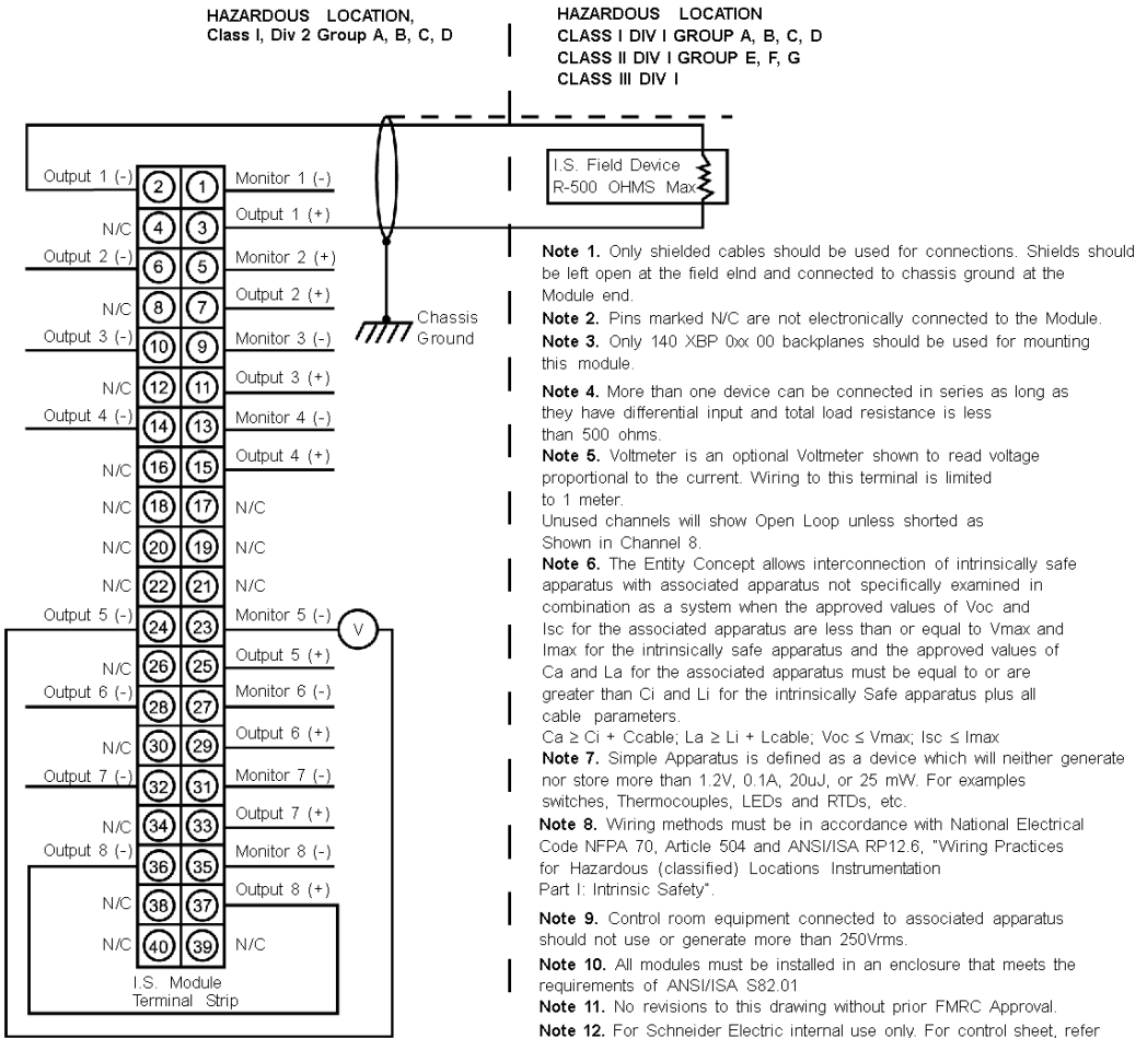
140 AIO 330 00 Wiring Diagram 31001364 Rev 01
