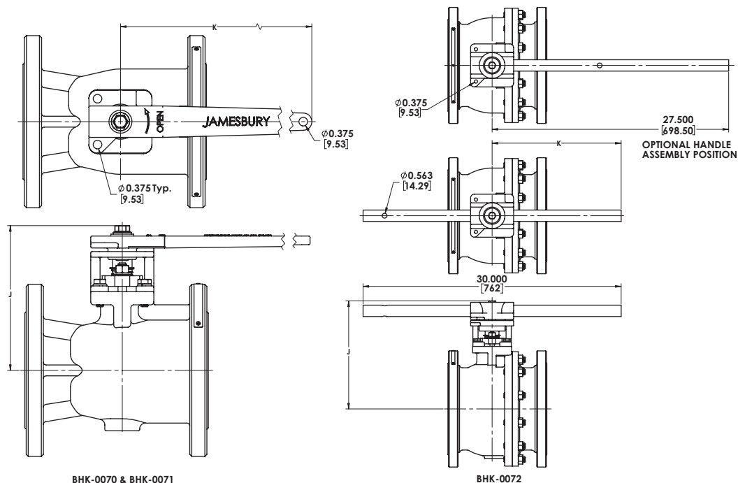
Series 7150 ASME Class 150 Approximate Dimensions - inches
