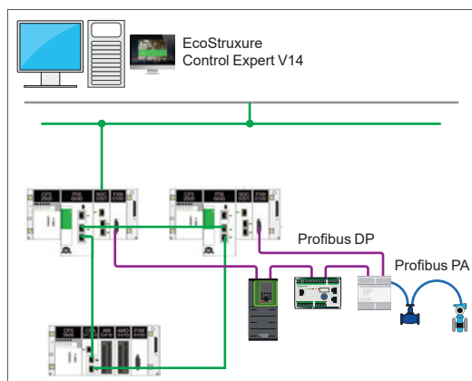
Redundant (HSBY) topology to connect the Profibus DP master X80 module to M580/X80 platforms with PMEPM0100
