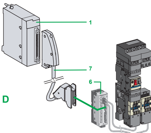
Example of connection to the TeSys Quickfit installation system
