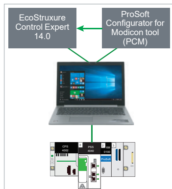
Interaction between EcoStruxure Control Expert, Prosoft Configurator for Modicon (PCM tool), and PMEPM0100 Profibus DP master X80 module
