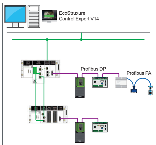
Standalone topology to connect Profibus DP master X80 module to M580/X80 platforms with PMEPM0100
