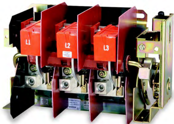
Figure 9 - Flange Mounted, Variable Depth Disconnect Switch — 9422TF1
