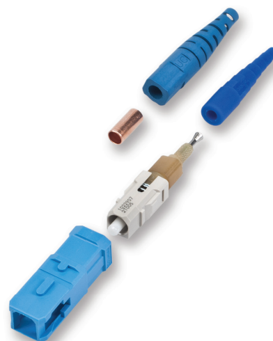
Part Number: 95-200-41
