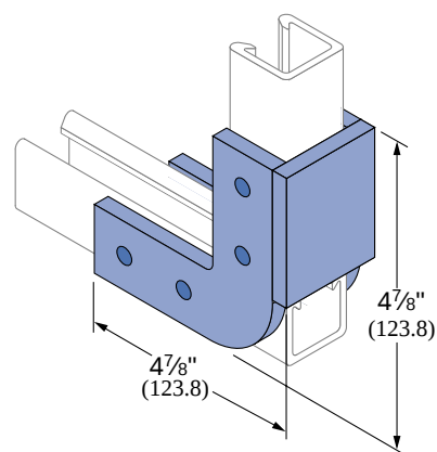
F50PU-1508 (1 1/2"), F50PU-2008 (1 5/8") Wt/100 pcs: 27 Lbs (12.2 kg)
