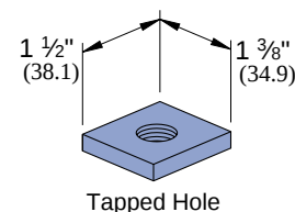
Tapped Hole
