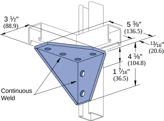
P1956 Wt/100 pcs: 230 Lbs (104.3 kg)
