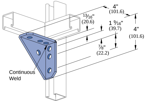
P2484W Wt/100 pcs: 134 Lbs (60.8 kg)
