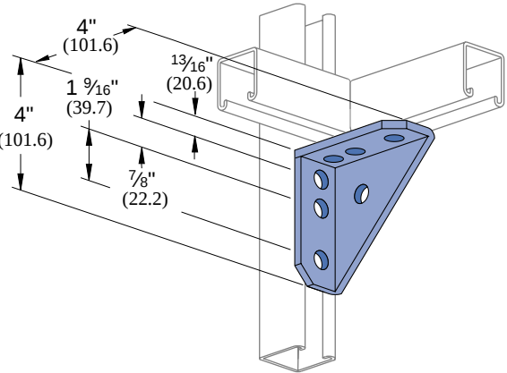
P2484 Wt/100 pcs: 134 Lbs (60.8 kg)
