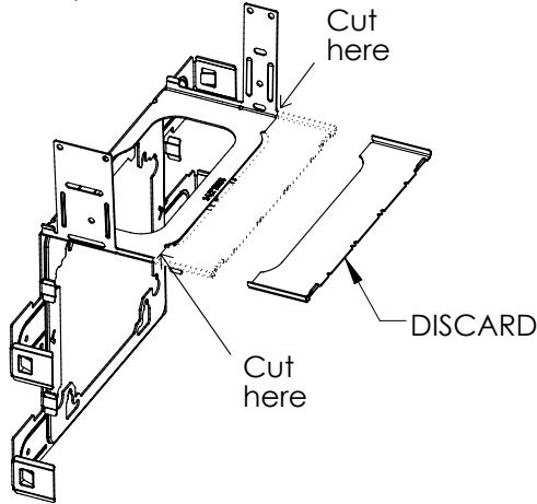
Step 1 2-1/2" studs
