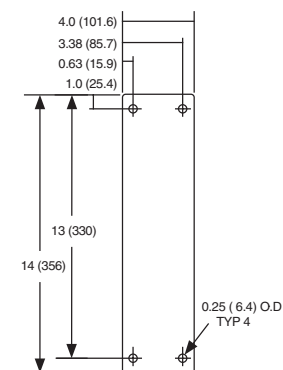
WPS/WPSA Vertical Mount Flange Front View
