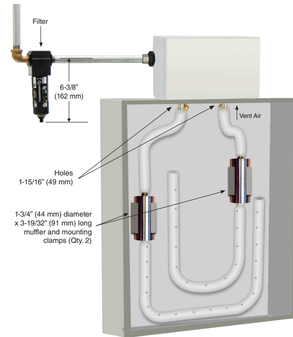
VORTEX A/C TYPE 4/4X (SHOWN TOP MOUNTED ON CUSTOMER'S ENCLOSURE)
