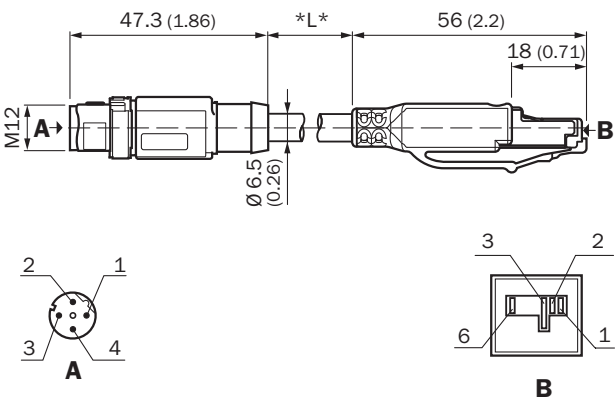
Dimensional drawing (Dimensions in mm (inch))
