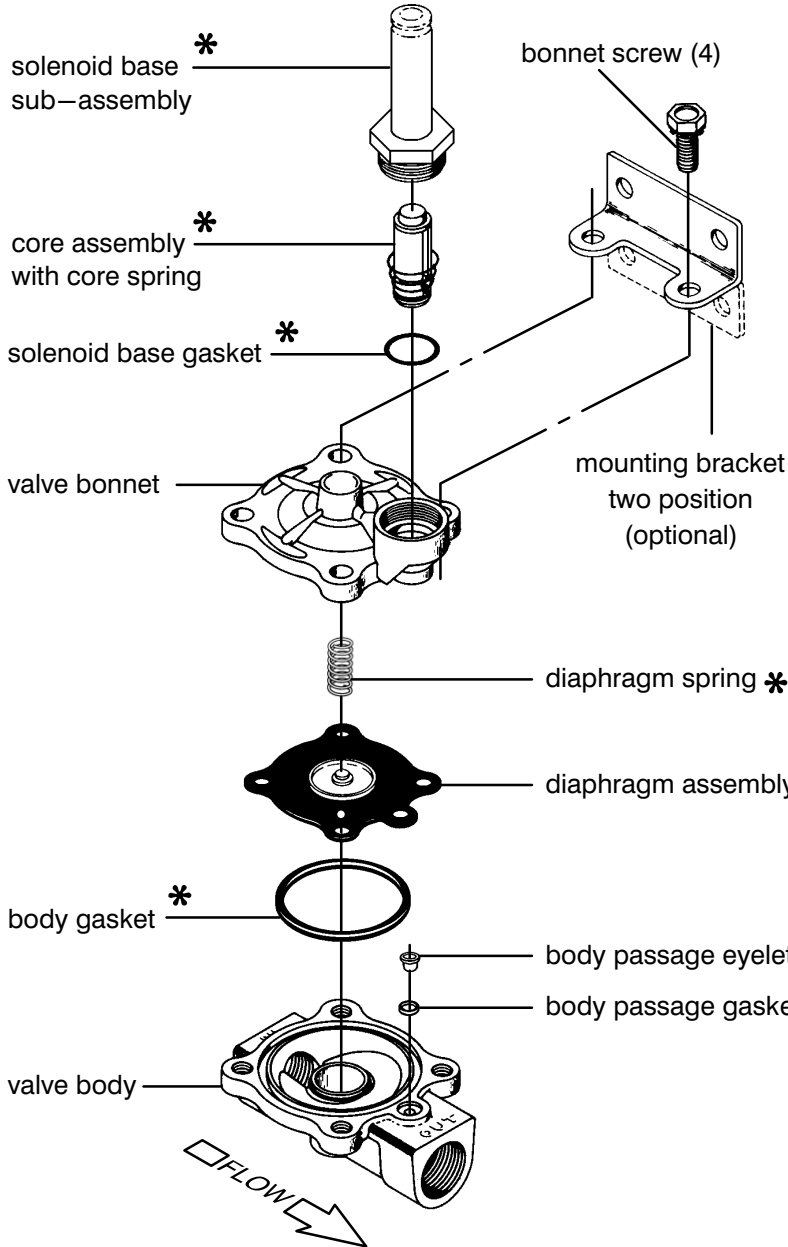
Figure 3. Series 8210 without solenoid, DC construction shown.
