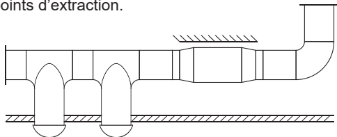
Figure 2. Installing / Instalación / Installation: TD - MIXVENT SERIES.
